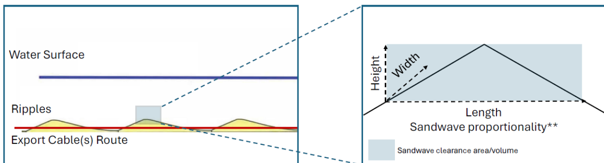
Figure 7: Sandwave profile
